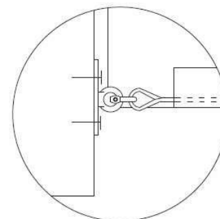
Fixture of curtain bottom with cable
