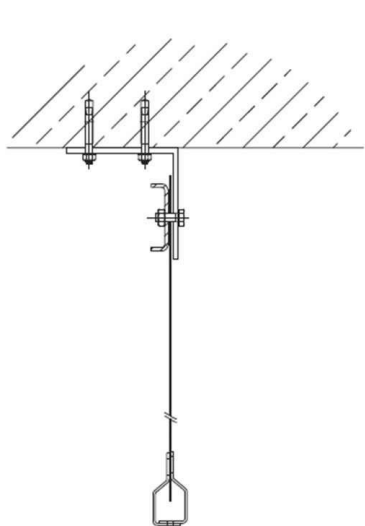
S type curtain installation under lintel, using angle profile
