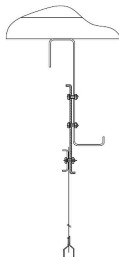
S type curtain installation to lintel
