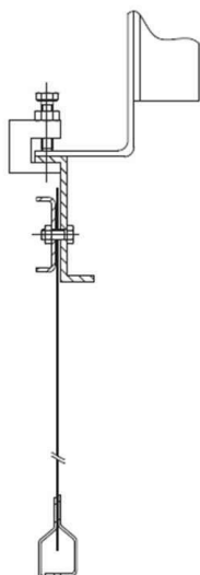
S type curtain installation to beam, using vice
